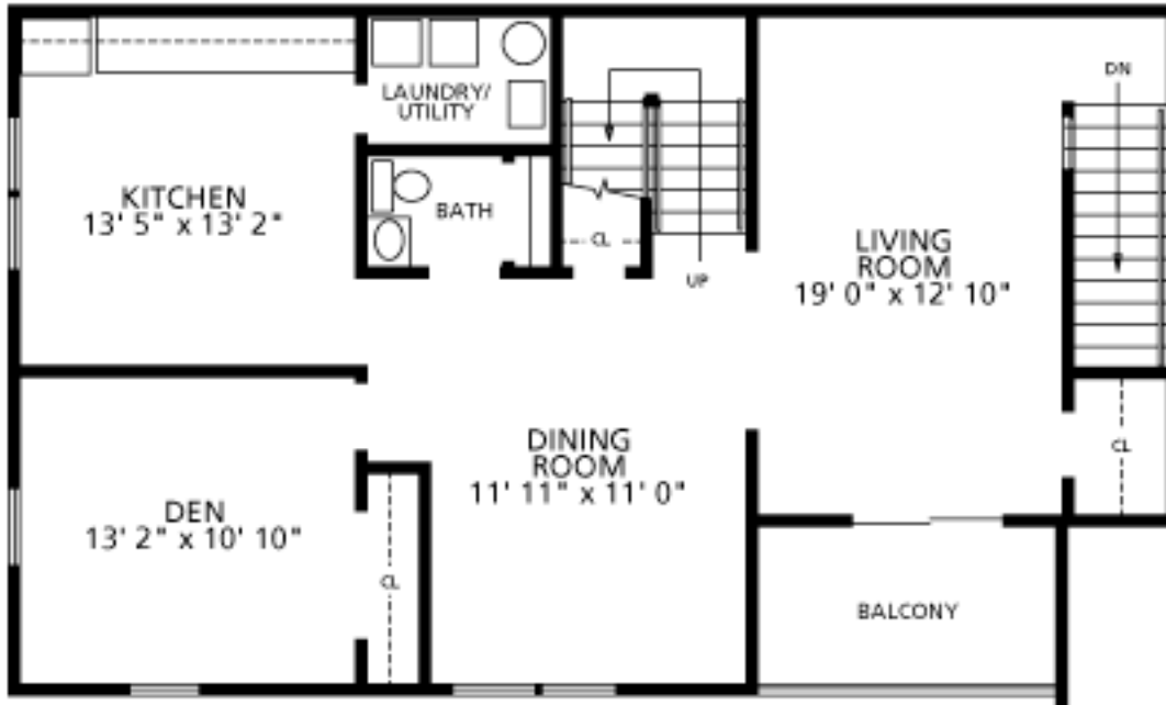
Three Bedroom Duplex Floor 1
