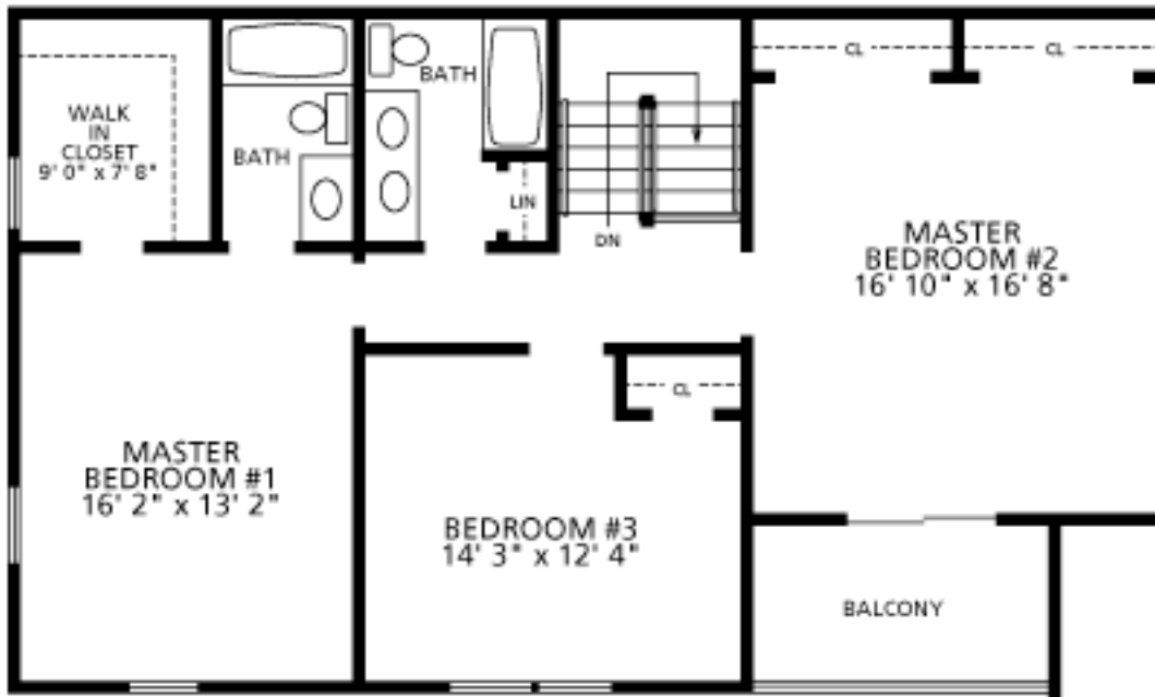
Three Bedroom Duplex Floor 2
